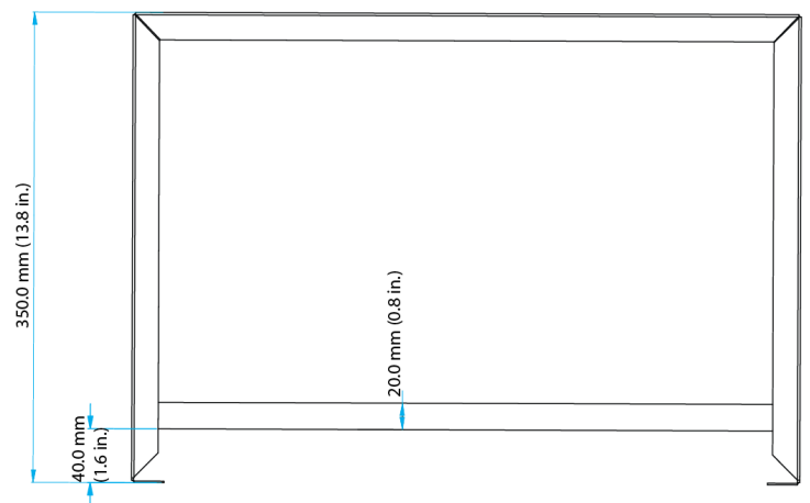
View looking down on the WALLMOUNT6
