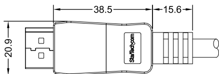
BACK VIEW
