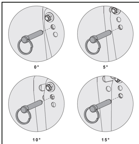
Adjustment Positions
